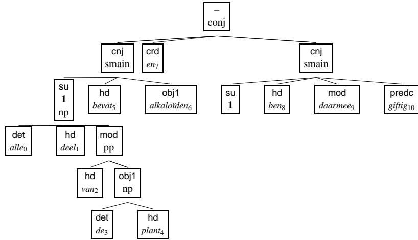
FIGURE 2 Dependency tree for (3-b)
