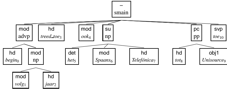
FIGURE 1 Dependency tree for (3-a)
